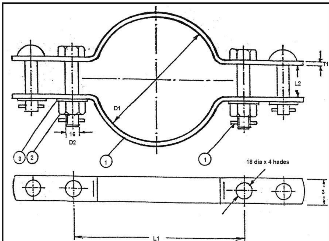
POLE MOUNTED STAY CLAMP (RAIL)
