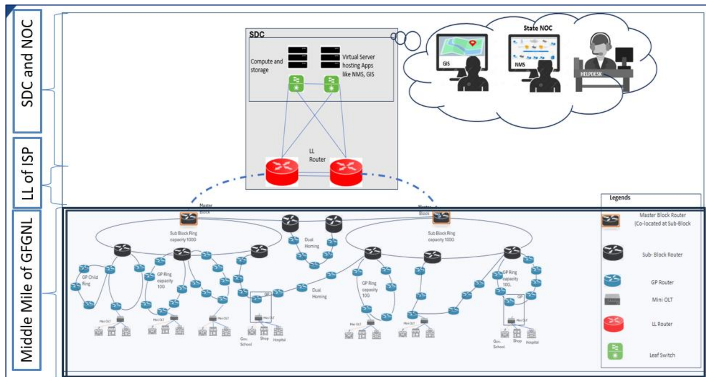
Drawing-A (Network Design BharatNet Phase-III)
